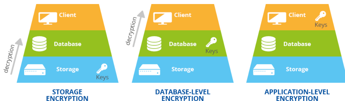
Figure 2: Database Encryption Options
